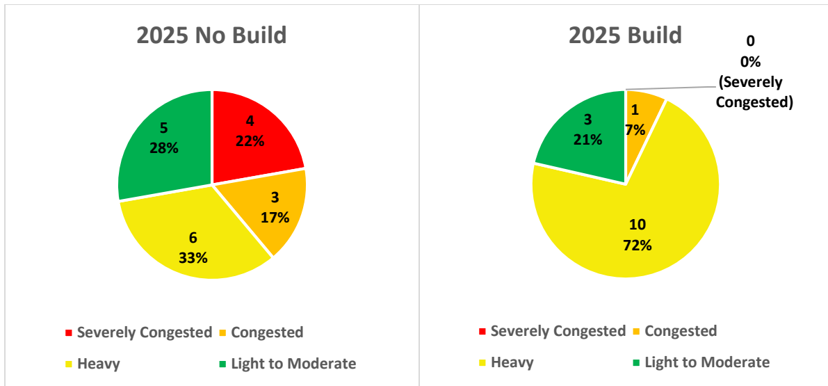
Figure 7-6: 2025 AM Freeway Segment Densities for I-495 Southbound GP Lanes
