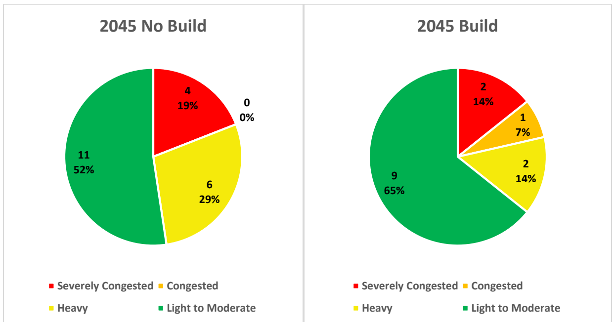
Figure 7-35: 2045 PM Freeway Segment Densities for I-495 Southbound
